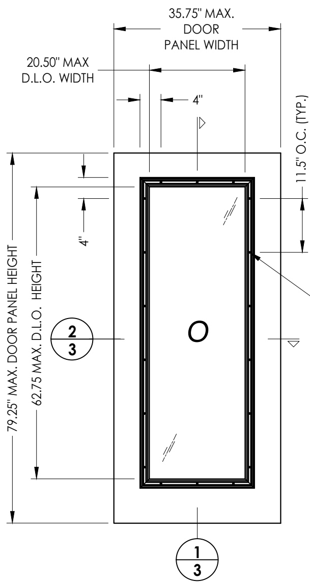
60 SIDELITE PANEL
