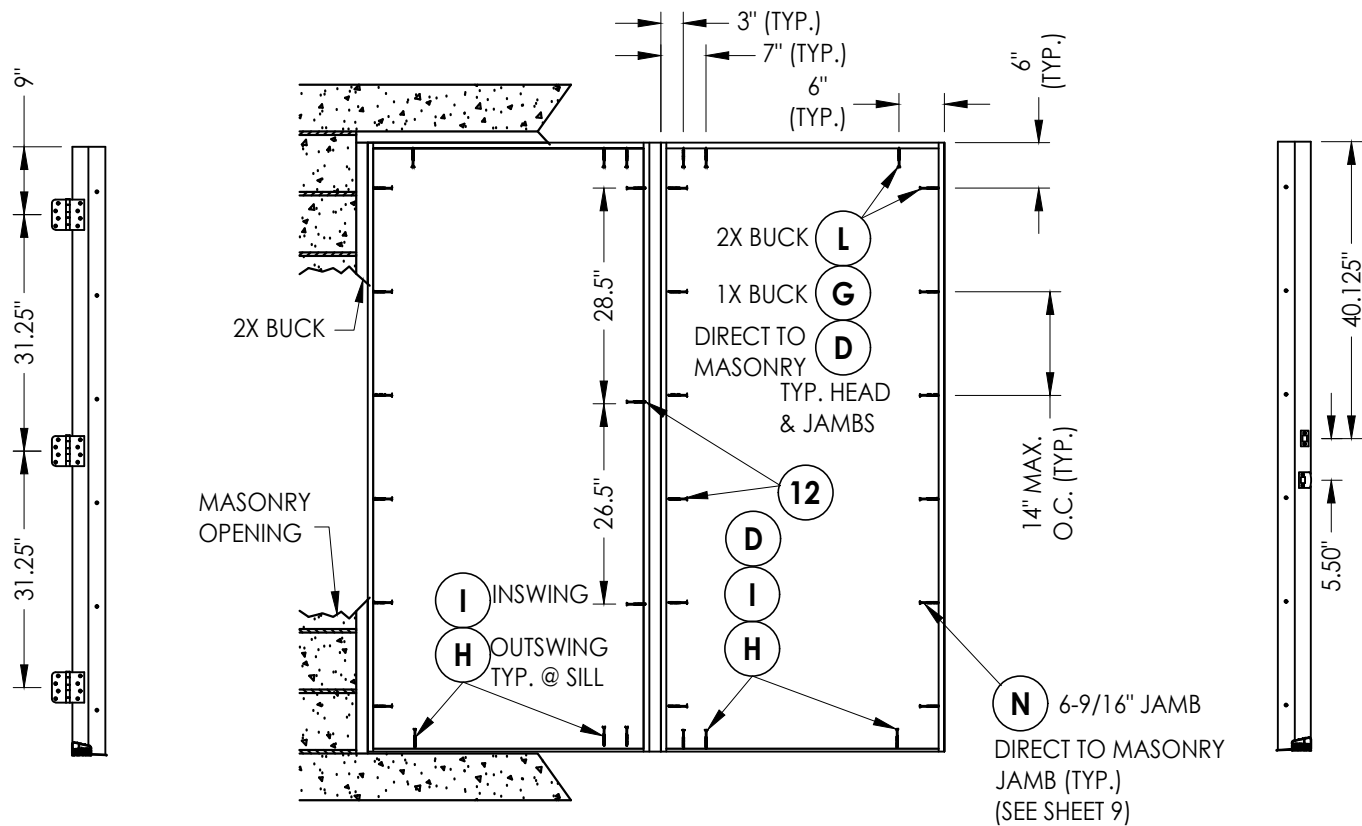
FRAME ANCHORING Masonry 2X buck construction
