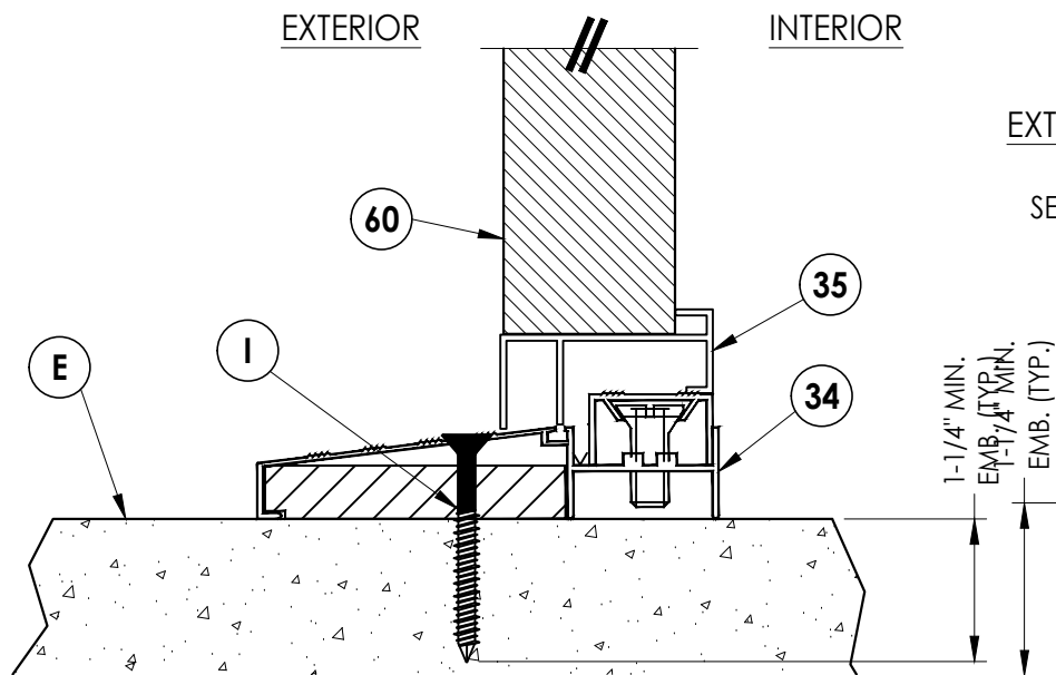
3 8 VERTICAL CROSS SECTION Inswing configuration
