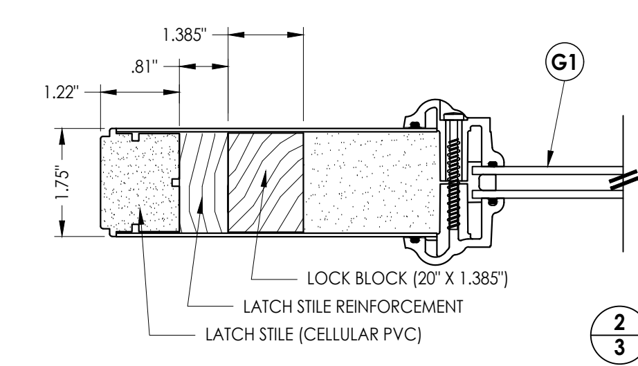
2 3 HORIZONTAL CROSS SECTION
